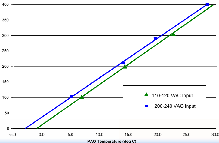
Figure 1 Cooling Performance of ThermoCube PAO PAO Coolant, 20 deg C Ambient
